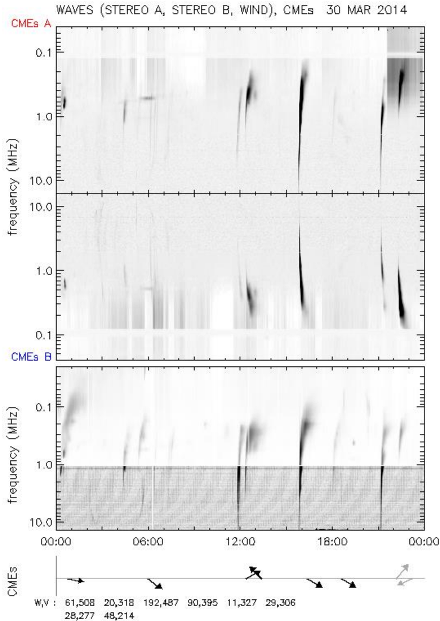
Fig. 3 – Radio emission as seen by STEREO A (first row), STEREO B (second row) and Wind (third row). Detected CMEs are shown in the last row.
