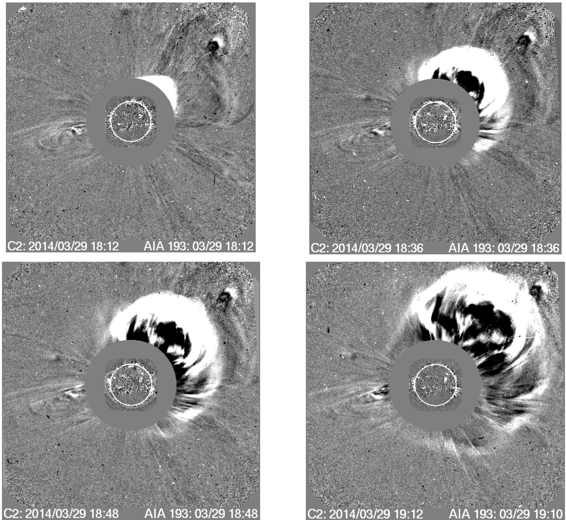
Fig. 2 – Running-differences of LASCO-C2 white-light images for the CME on March 29, 2014. Images from http://cdaw.gsfc.nasa.gov/CME_list/ .
