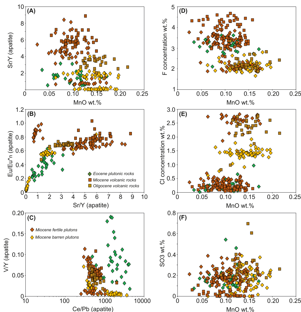
Fig. 7. \text{Sr}/\text{Y} vs \text{MnO} (wt%) (A), \text{Eu}/\text{Eu}^*_{(n)} vs \text{Sr}/\text{Y} (B), \text{V}/\text{Y} vs \text{Ce}/\text{Pb} (C), fluorine (wt%) vs \text{MnO} (D), chlorine (wt%) vs \text{MnO} (E) and \text{SO}_3 (wt%) vs \text{MnO} (F) compositional variation diagrams for apatite grains from southeastern UDMB igneous rocks. \text{MnO} , F, Cl and \text{SO}_3 have been analyzed by Electron Microprobe whereas trace elements such as Eu, Gd, Sm, V, Y, Ce and Pb have been analyzed using Laser Ablation Inductively Coupled Plasma-Mass Spectrometry (see text for explanations).
