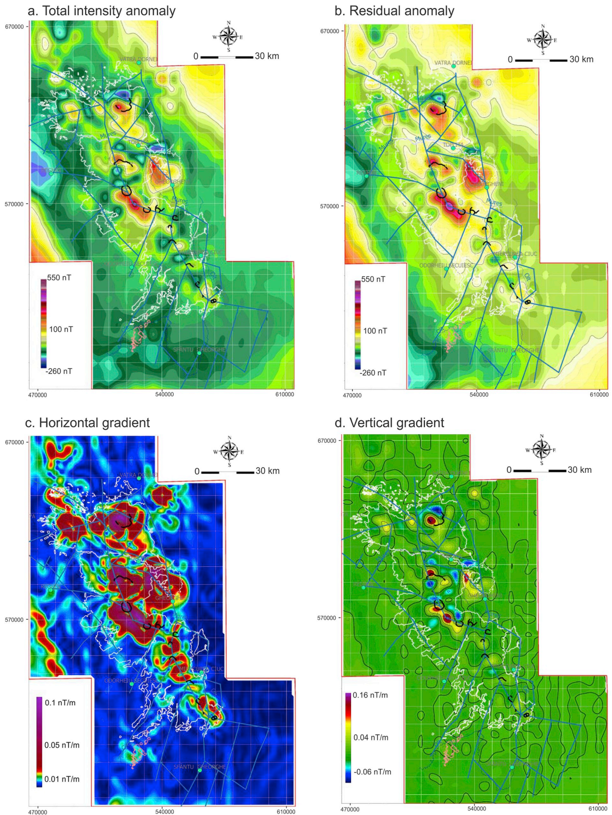
Fig. 5. Geophysical magnetic maps: (a) Total intensity anomaly, (b) residual magnetic anomaly, (c) horizontal gradient of the residual magnetic anomaly, (d) vertical gradient of the residual magnetic anomaly. Geomagnetic reference field IGRF12, reference altitude 2500 m, Krigging interpolator with cell size of 5 \times 5 km, DTM map scale 1:100000, projection system Stereo 1970, altitude datum Black Sea 1975.
