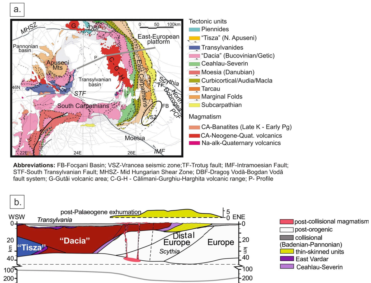
Fig. 1. (a) Location of the Călimani-Gurghiu-Harghita (CGH) volcanic range within the tectonic map of the Romanian Carpathians (compiled from Mațenco et al., 2010; Săndulescu, 1984; Schmid et al., 2008). (b) Interpretative cross-sections through the post-collisional environment of the CGH, including magmatic system (after Mațenco et al., 2010).
