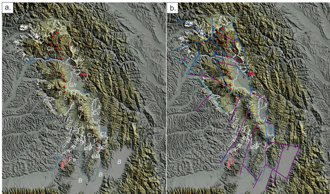
Fig. 3. (a) Morphological map of the CGH: Ca, Călimani; F-L, Fâncel-Lăpușna; ST, Seaca-Tătarca; B, Borzont; S, Șumuleu; CF, Ciurani-Fierăstraie; O, Ostorog; IC, Ivo-Cocoizaș; V, Vârghiș; L, Luci-Lazu; Cu, Cucu; P, Pilișca; Ci, Ciomadul and Pe, Peșani basaltic volcanic field; intra-mountain sedimentary basins: Bi, Bilbor; Bo, Borsec; Gh, Gheorgheni; UC, Upper Ciuc; LC, Lower Ciuc; B, Brașov; Ba, Baraolt; DM - Ditrau syenite Massive; (b) Tectonic features of the CGH (compiled after Seghedi et al., 1994; Fielitz and Seghedi, 2005; Krézsek and Bally, 2006; Szakács and Krezsék, 2006). The fault represented in light blue is associated with salt diapirs; deep blue color corresponds to strike slip faults; violet corresponds to normal faults. (For interpretation of the references to color in this figure legend, the reader is referred to the web version of this article.)
