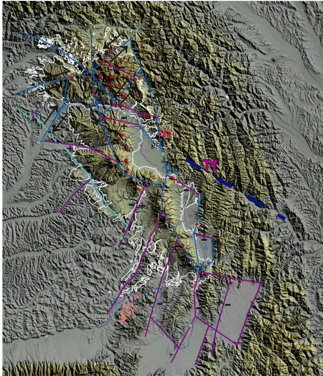
Fig. 6. The configuration of normal and transcurrent faults and fractures. It governed the evolution of Late Miocene–Quaternary volcanism and basin subsidence along a transensional corridor in the CGH range. The volcanic centers are concentrated along the western margin of this corridor (modified after Fielitz and Seghedi, 2005). All the details and signs are the same as those explained in Fig. 3a, b.
