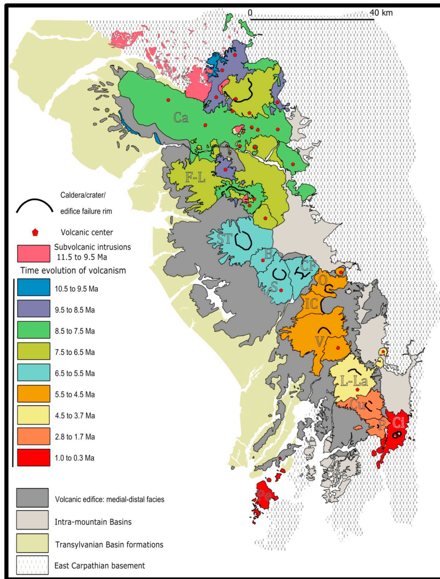
Fig. 7. The evolution in space and time of the main composite volcanoes along the CGH range (age data after Pécskay et al., 1995, 2006; Molnár et al., 2019). Name abbreviation of the volcanoes as in the Fig. 3a.
