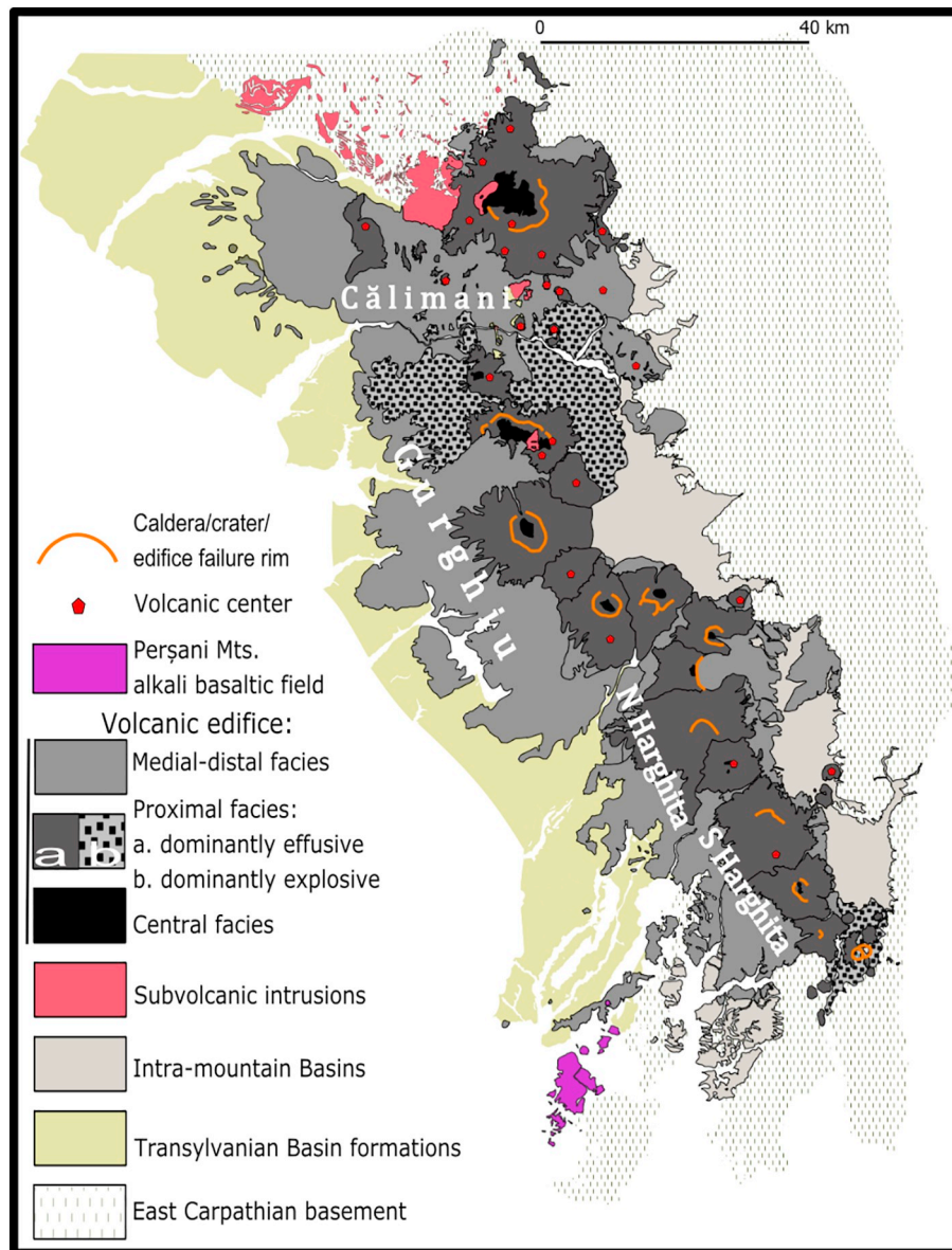
Fig. 2. Simplified volcanic facies map of the Călimani-Gurghiu-Harghita volcanic range (modified from Szakács and Seghedi, 1995).
