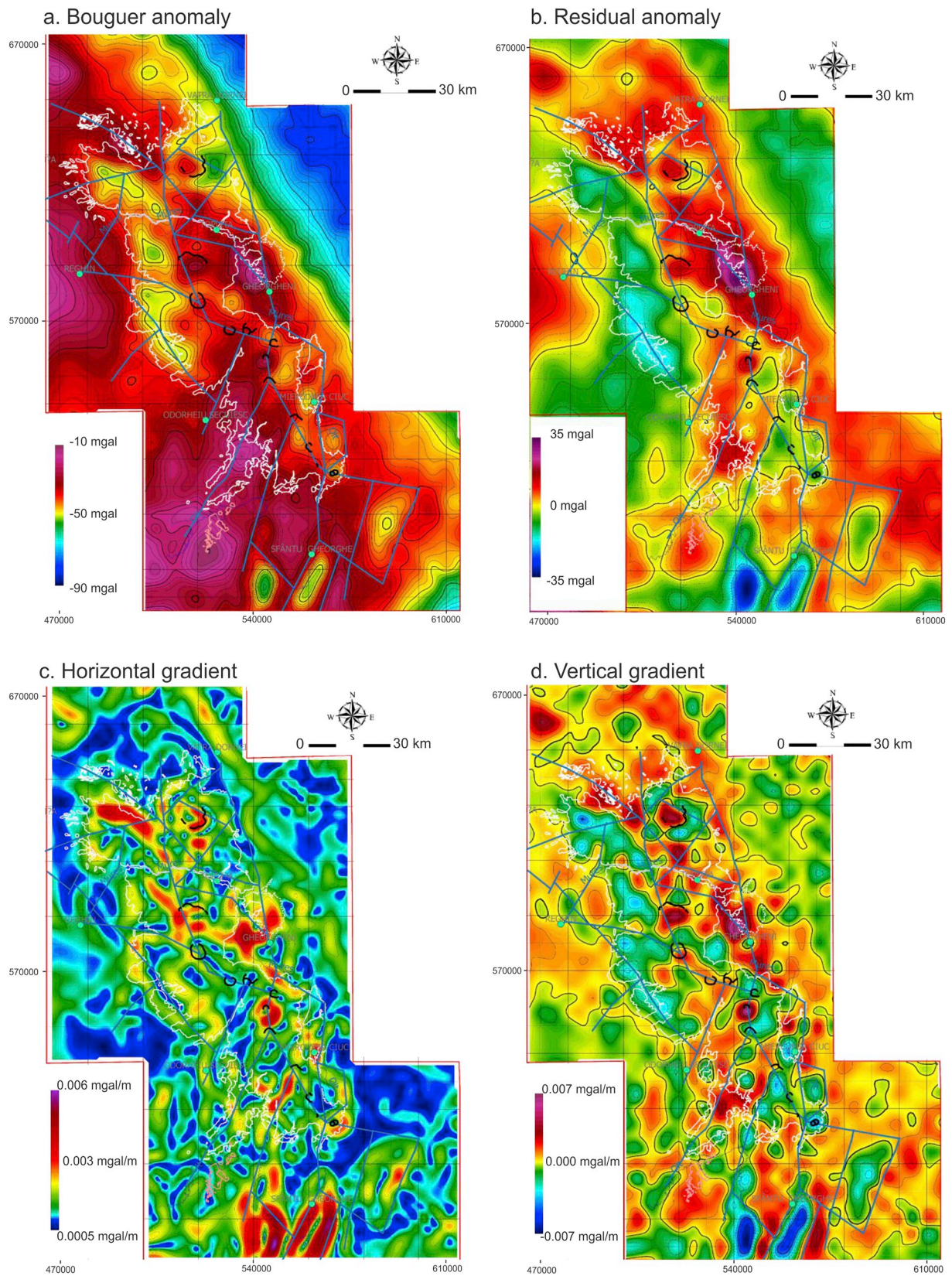
Fig. 4. Geophysical gravity maps: (a) Bouguer anomaly, (b) residual gravity anomaly, (c) horizontal gradient of the residual gravity anomaly, (d) vertical gradient of the residual gravity anomaly. Bouguer correction radius is 20 km, Krigging interpolator with cell size of 5 \times 5 km, DTM map scale 1:100000, projection system Stereo 1970, altitude datum Black Sea 1975.
