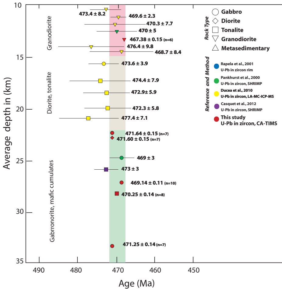
Figure 2. U-Pb ages projected onto an averaged one-dimensional depth section. Because the thickness of the distinct compositional domains is not uniform along the strike of the arc section, it was necessary to create an average thickness and project the data onto that. Relative depths and spacing are preserved, but actual depths will vary for the deepest samples. Vertical colored bar of ~4 m.y. bounds the new high-precision chemical abrasion–thermal ionization mass spectrometry (CA-TIMS) data and overlaps uncertainties in all available data (LA-MC-ICP-MS—laser ablation–multicollector–inductively coupled plasma–mass spectrometry). We take the 4 m.y. range as the duration of igneous activity that formed the arc section. Errors are given at 2\sigma .
