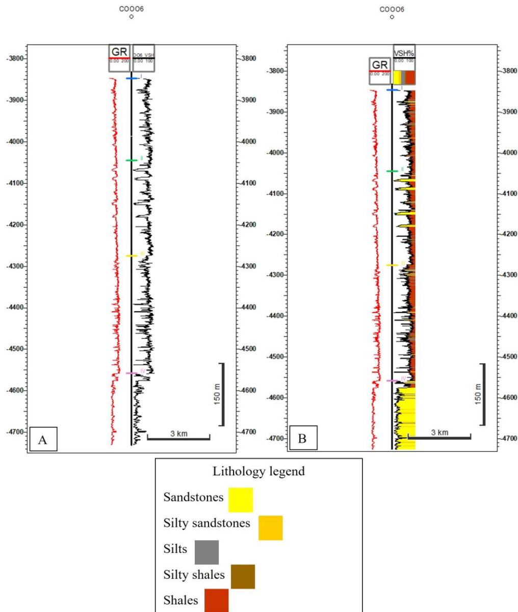
Fig. 4 – V_{\text{sh}} curve obtained by processing the gamma ray log (A) and the associated lithology that was delineated using multiple cut-off values (0–25 for sands/sandstones, 25–35 for silty sands/silty sandstones, 35–55 for silts, 55–60 for silty shales, 60–100 for shales).
