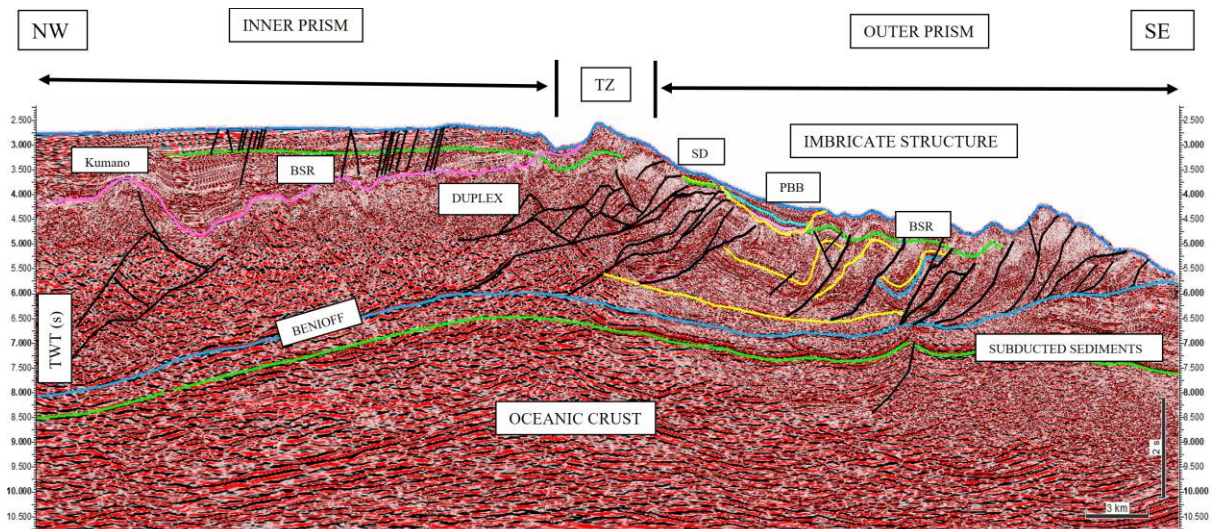
Fig. 2 – Regional TWT seismic cross section along the Nankai accretionary prism showing the main tectonic elements.
